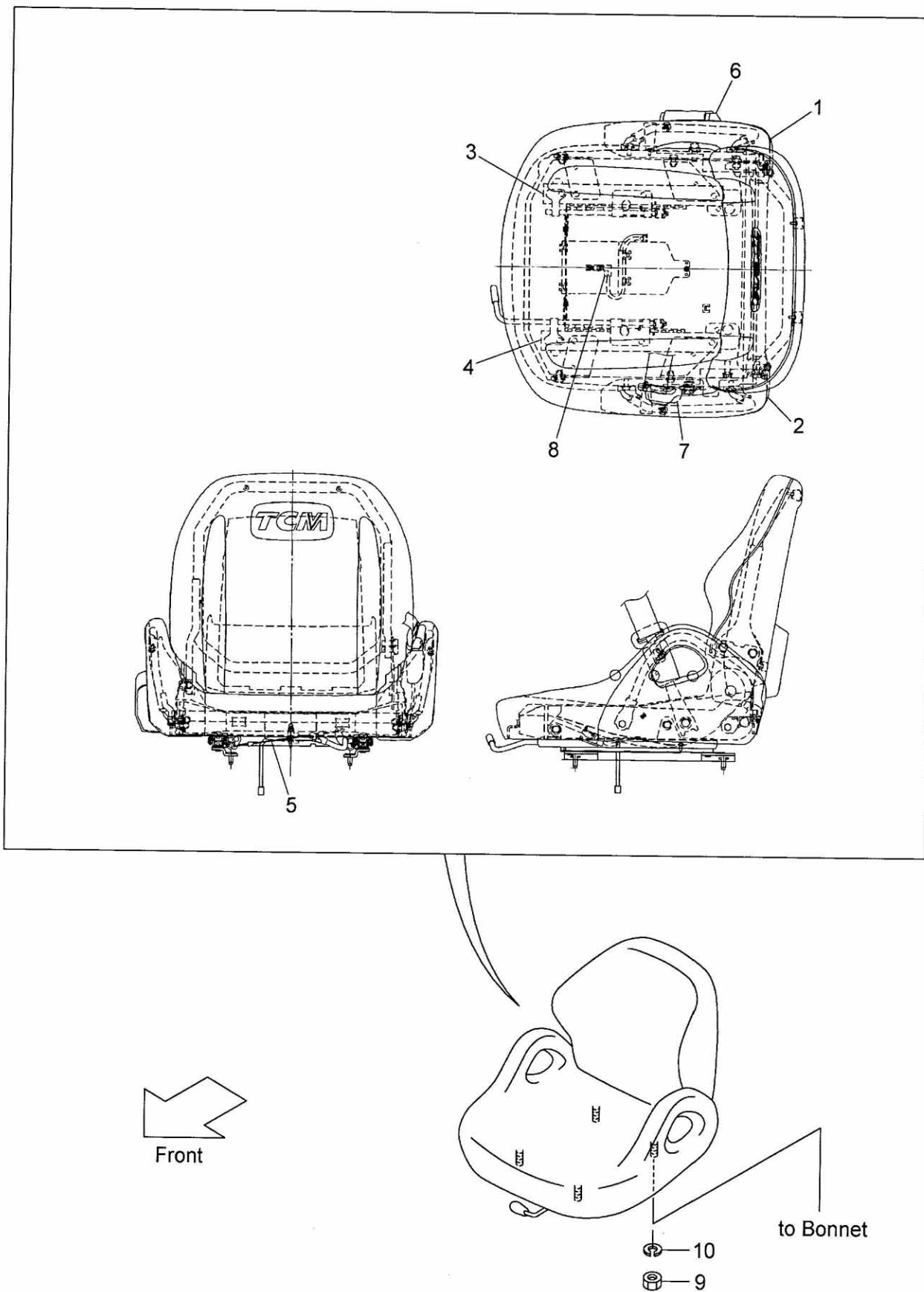
FIG.138 SEAT [EXB/SIL/HGL][EXC/SIL/HGL][EXK/SIL/HGL] (F7C368D0) シート
