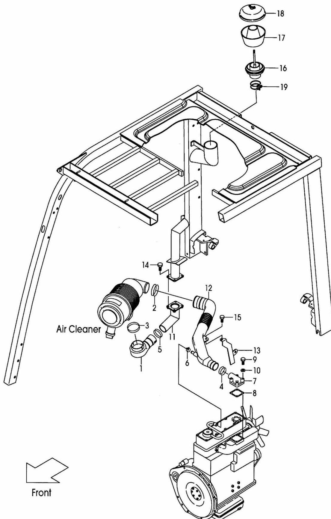
FIG.4 AIR DUCT [CAKB] (F7C31080) エア・ダクト
