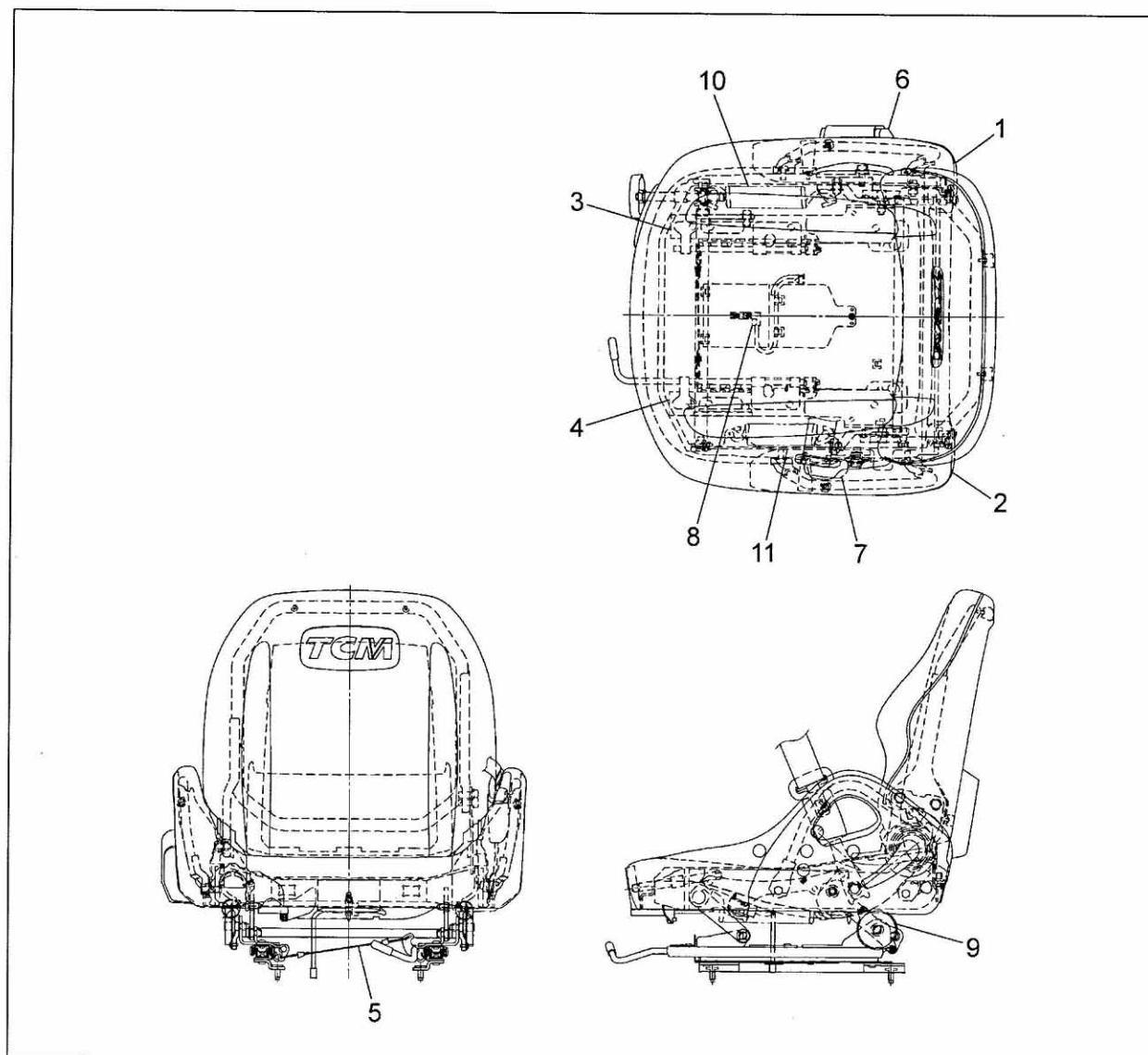
FIG.137 SEAT [EXB/SIL][EXC/SIL][EXK/SIL] (F7C368B0) シート
