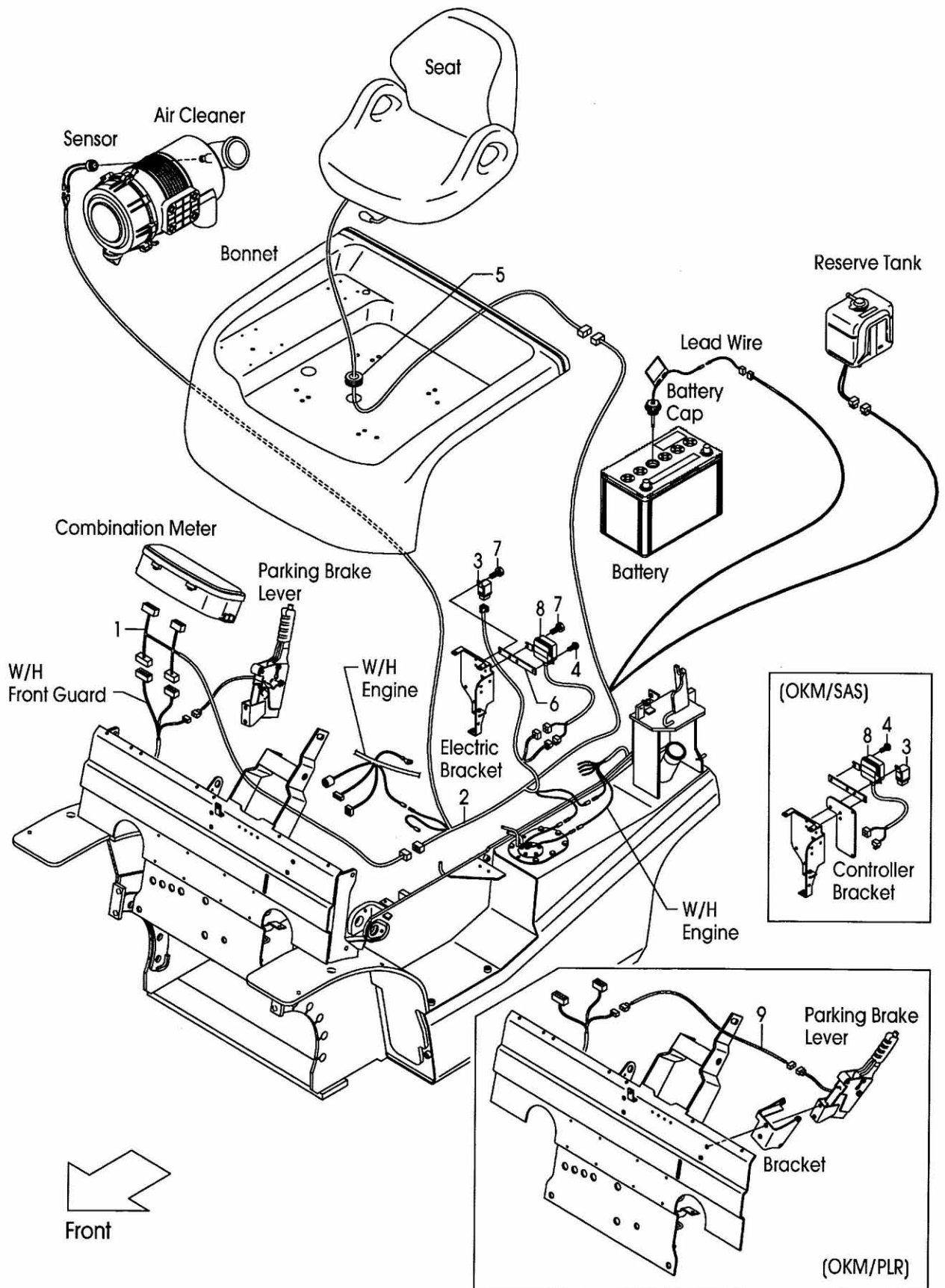
FIG.53 OK MONITOR [OKM] (F7C326J0) OKモニタ
